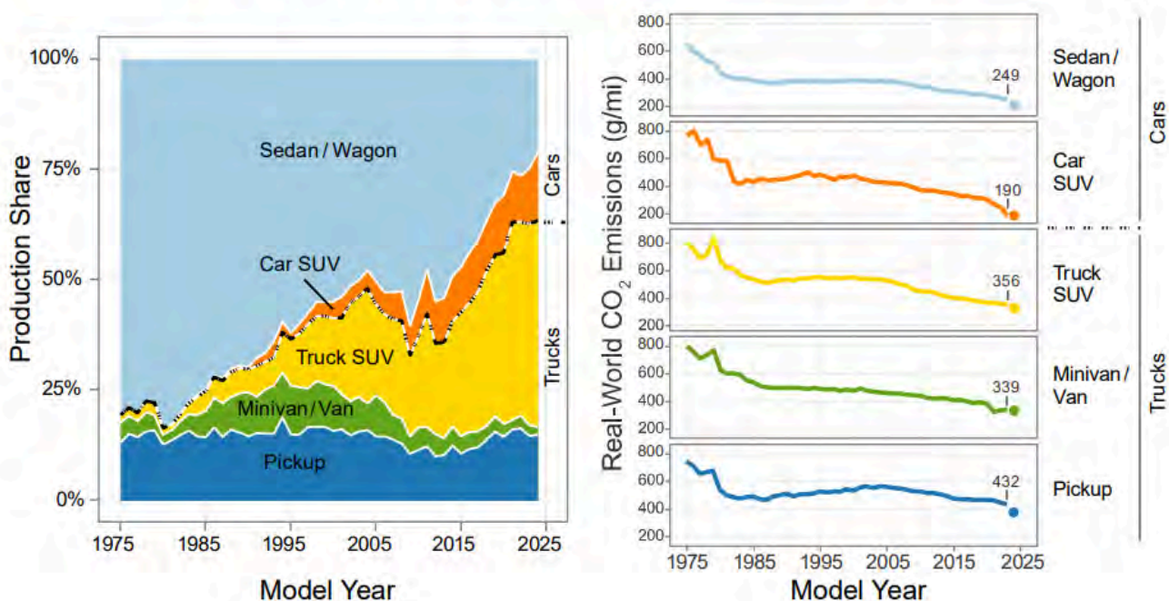
Production Share and Estimated Real-World CO 2 Emissions
